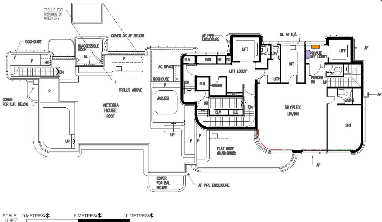
Mansion 1 5/F Floor Plan Mansion 1 5樓平面圖
